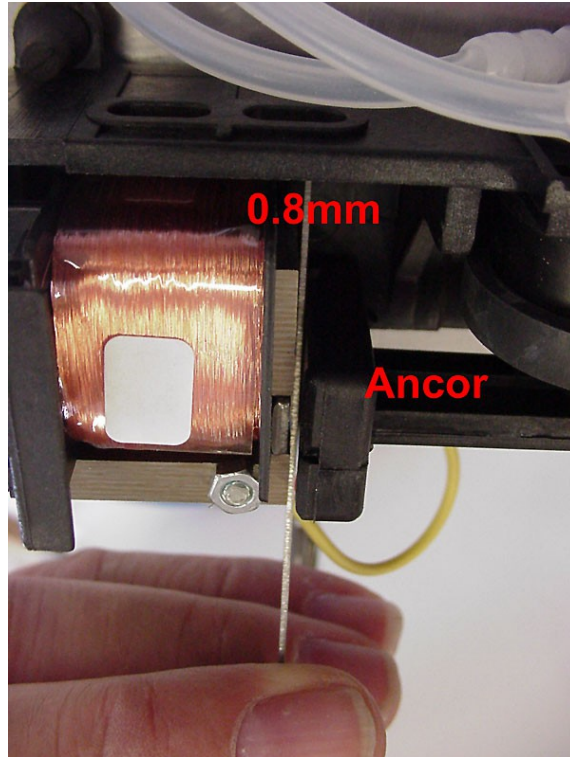
Gap between Magnet and Swing-Ancor
