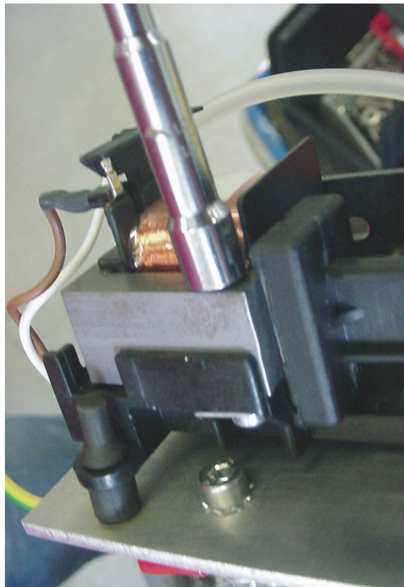
Attachment screw. Magnet may be shifted when loosen attachment screw.
